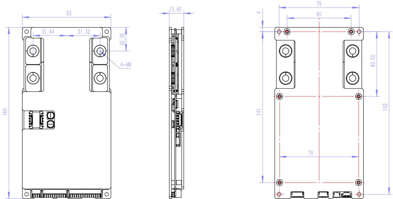
JK-BD6A24S-15PD外形尺寸
