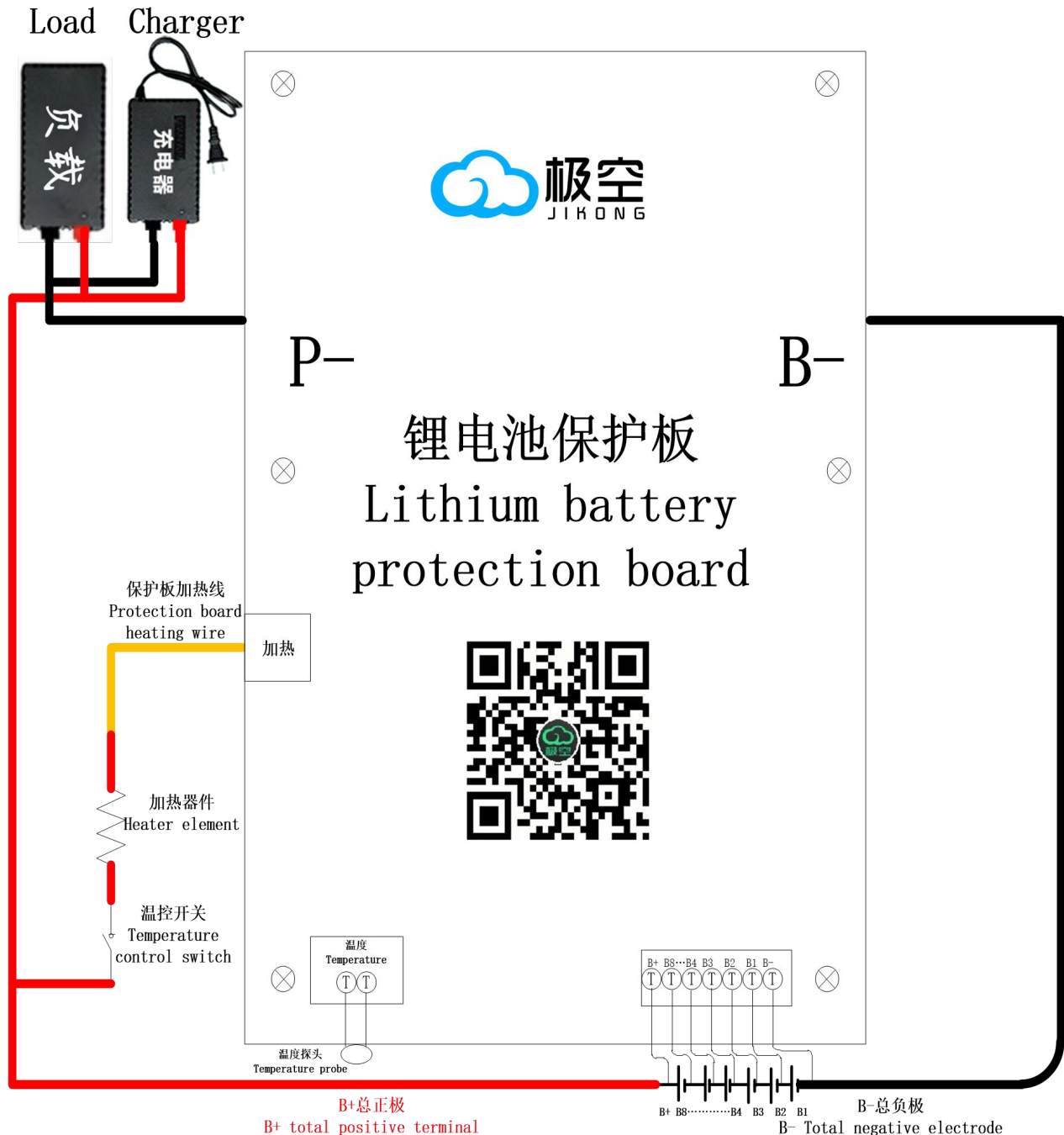
JK-BD6A8S-10P接线图
